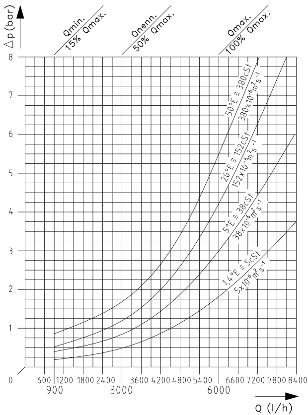
B – GHG – E – SAE 1"
