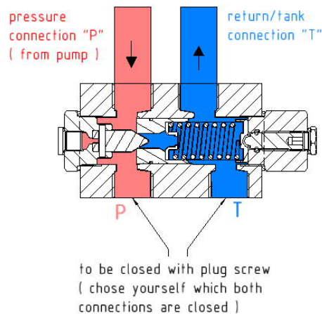
Fig.2 One pipe system
