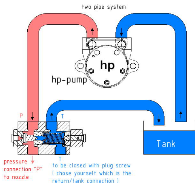
Fig.3 Two pipe system
