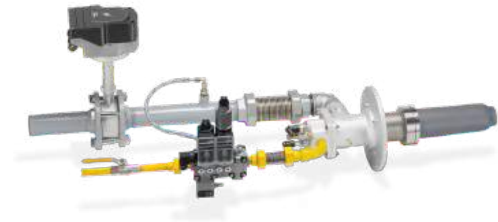
Gas adjusting cock GEH in a burner line
